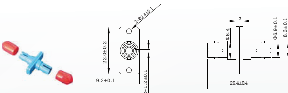
Footprint Simplex Plastic Type
