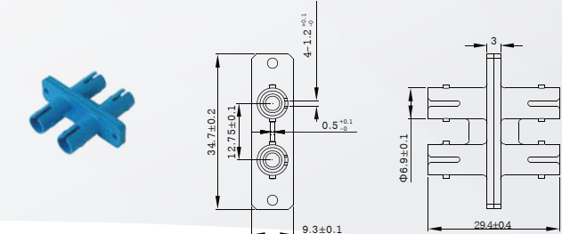
Footprint Duplex Plastic Type
