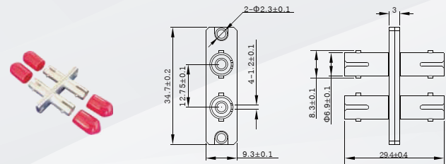
Footprint Duplex Metal Type
